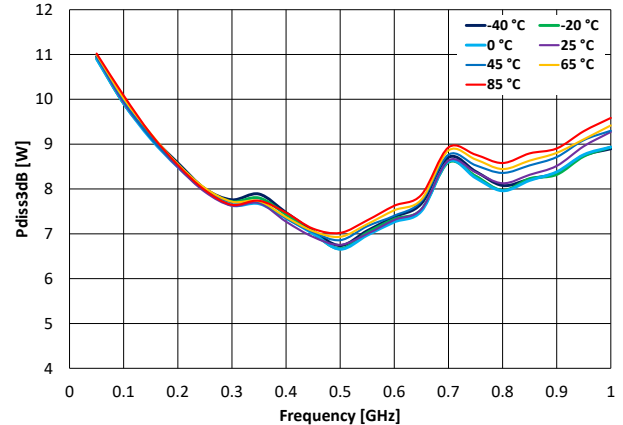
Pdiss3dB Over Temperatures
