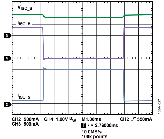
Figure 27. Load Transient. I_{ISO\_sx} Load = 300 mA to 1500 mA to 300 mA, EN\_CHG = High , ILIM[3:0] = 0110 (Binary) = 500 mA
