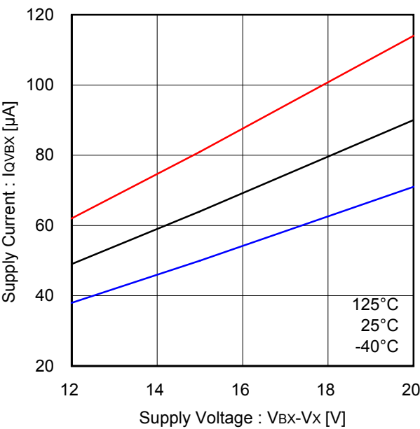
Figure 17. Quiescent Current (High Side Driver, Each Phase)
