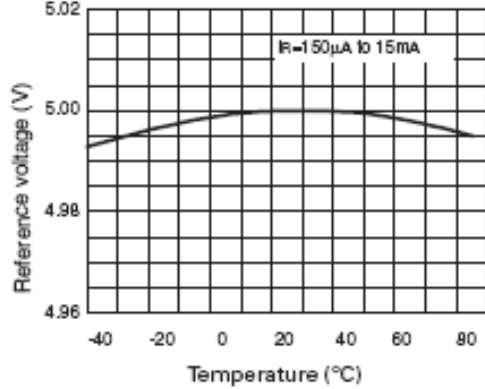
Temperature Drift
