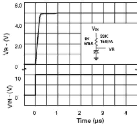
Transient Response (Repetitive Pulse)
