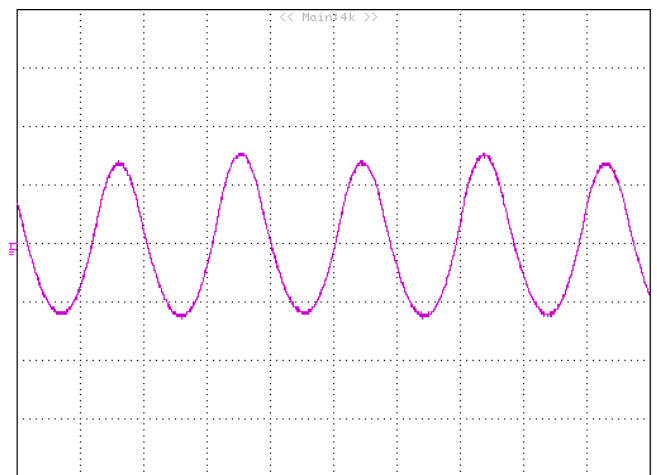
Figure 11: Input Terminal Ripple Current, i_c , at full rated output current and nominal input voltage with 12\mu H source impedance and 100\mu F electrolytic capacitor (1A/div, 2\mu s /div).
