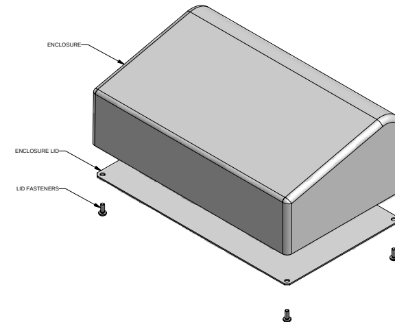
ENCLOSURE ASSEMBLY
