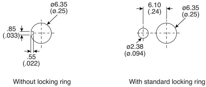
Panel Mounting
