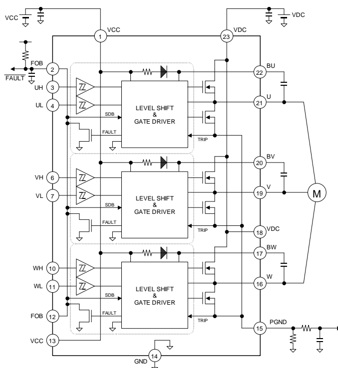
Figure 2. Block Diagram
