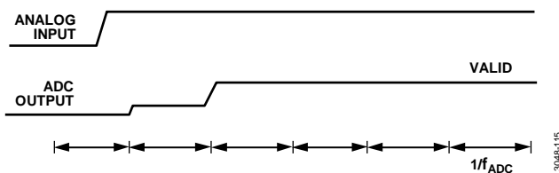
Figure 105. Step Change on the Analog Input, Sinc^3 + Sinc^1 Filter
