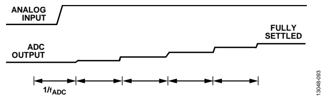
Figure 83. Asynchronous Step Change in the Analog Input
