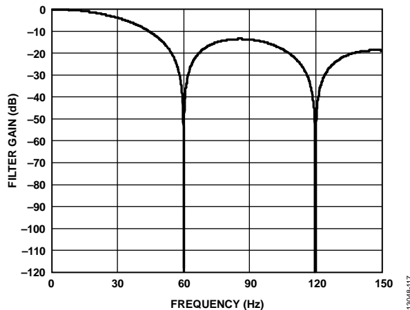
Figure 107. 60 Hz Rejection
