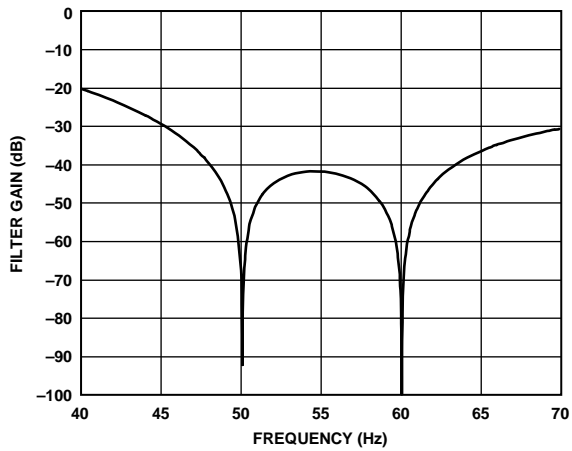
Figure 111. Zoom in 40 Hz to 70 Hz, 27.27 SPS Output Data Rate, 36.67 ms Settling Time
