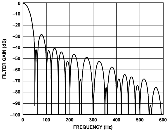
Figure 110. DC to 600 Hz, 27.27 SPS Output Data Rate, 36.67 ms Settling Time
