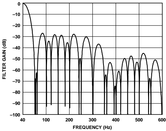
Figure 112. DC to 600 Hz, 25 SPS Output Data Rate, 40 ms Settling Time
