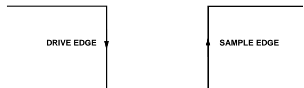
Figure 65. SPI Mode 3, SCLK Edges
