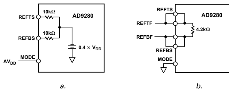
Figure 1. Equivalent Input Load
