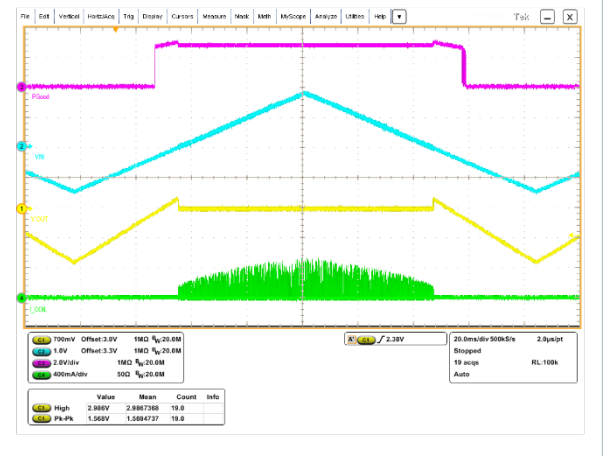
Figure 9. 100% mode, V_{OUT} = 3.0\text{ V}
