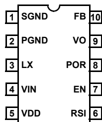
EL7536 (10 LD MSOP) TOP VIEW
