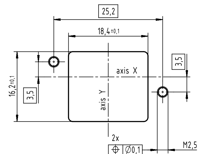
panel cutting
