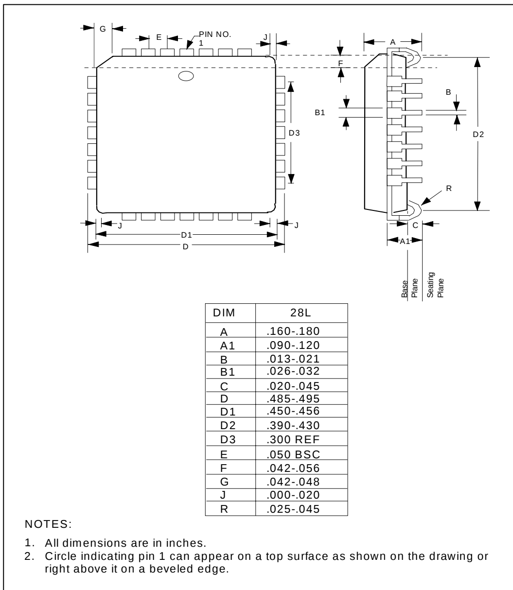
FIGURE 25 - 28 PIN PLCC PACKAGE DIMENSIONS
