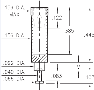
0389-X-15-XX-08-XX-10-0 Swage mount in .094 hole
