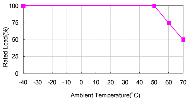
Derating curve:
