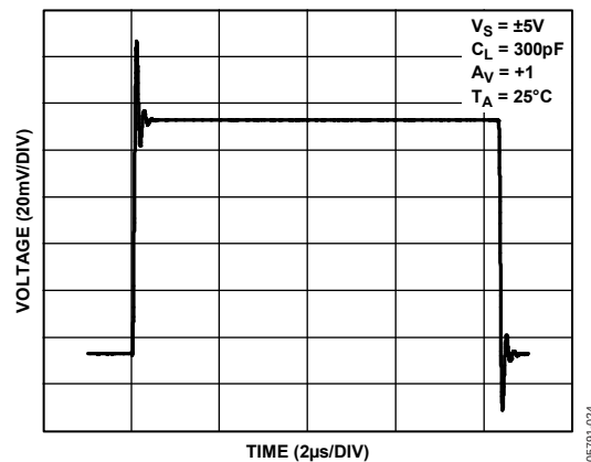
Figure 18. Small Signal Transient Response, V_S = \pm 5 V
