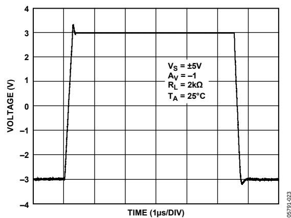
Figure 17. Large Signal Transient Response, V_S = \pm 5 V
