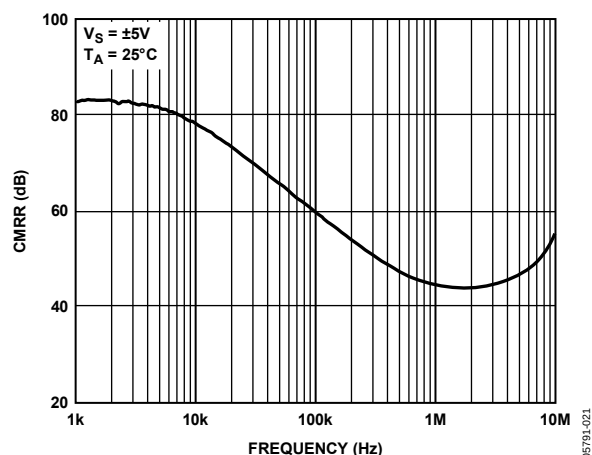
Figure 16. Common-Mode Rejection Ratio vs. Frequency, V_S = \pm 5 V
