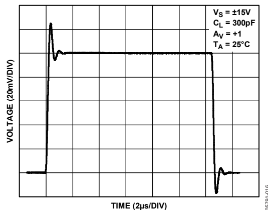
Figure 15. Small Signal Transient Response, V_S = \pm 15 V
