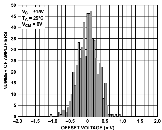
Figure 7. Input Offset Voltage Distribution, V_S = \pm 15 V
