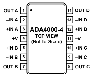
Figure 6. 14-Lead TSSOP (RU-14)
