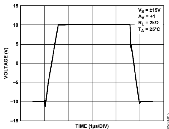
Figure 14. Large Signal Transient Response, V_S = \pm 15\text{ V}
