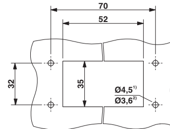
Mounting cutout
