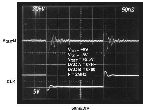
Figure 24. Digital Feedthrough
