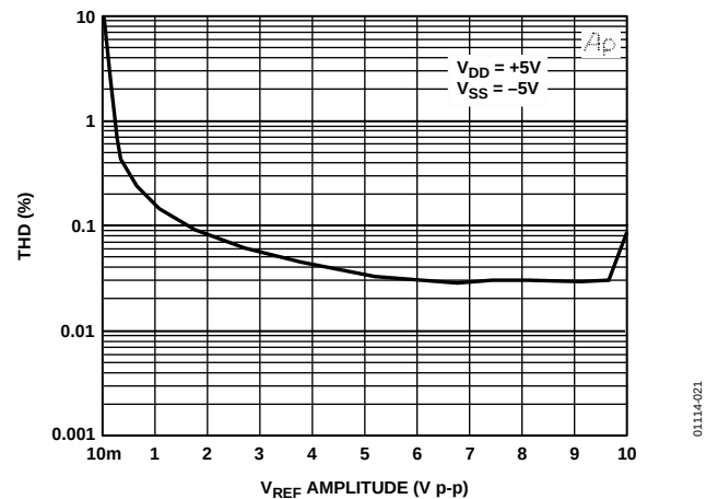
Figure 21. THD vs. Reference Input Amplitude
