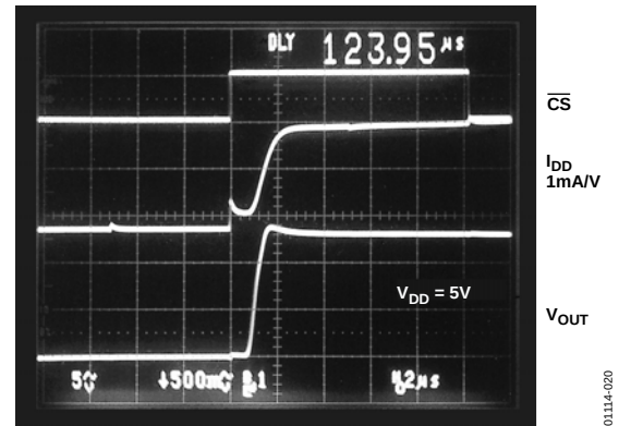
Figure 20. Shutdown Recovery Time (Wakeup)
