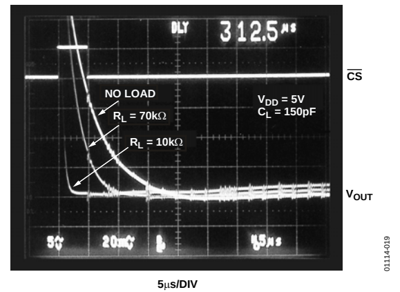
Figure 19. Time to Shutdown
