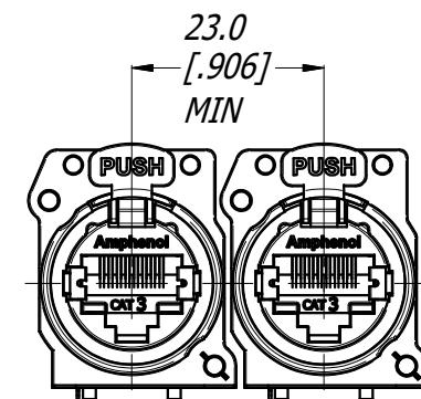
MIN MOUNTING PITCH 1:1
