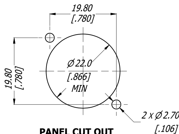
PANEL CUT OUT 3:2 (CONNECTOR FRONT VIEW)
