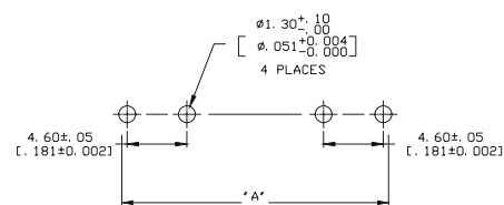
RECOMMENDED MOUNTING PATTERN
