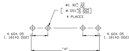
RECOMMENDED MOUNTING PATTERN
