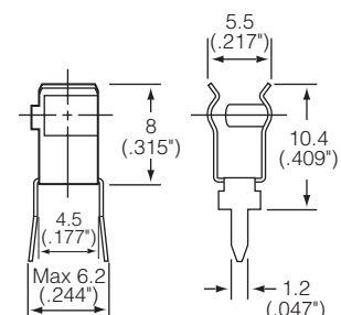
Mounting Dimensions for 445/030/520 Series
