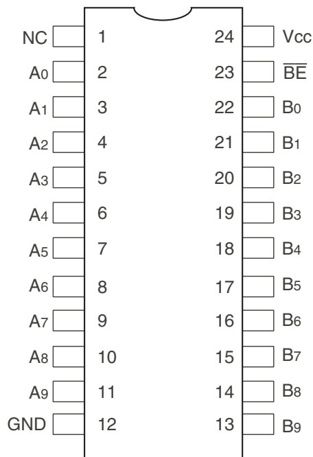
QSOP/ TSSOP TOP VIEW
