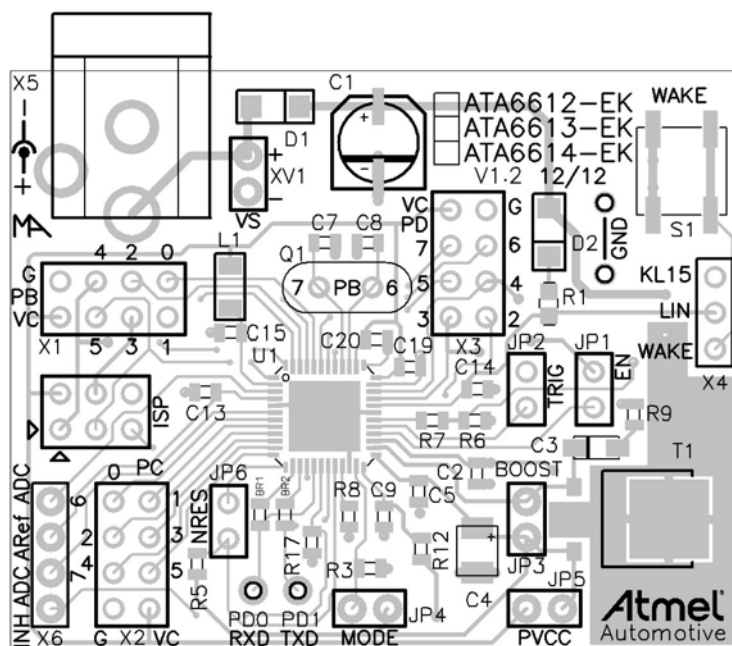
Figure 7-2. Atmel ATA6612/ATA6613/ATA6614 Board Component Placement; Top Side, Top View
