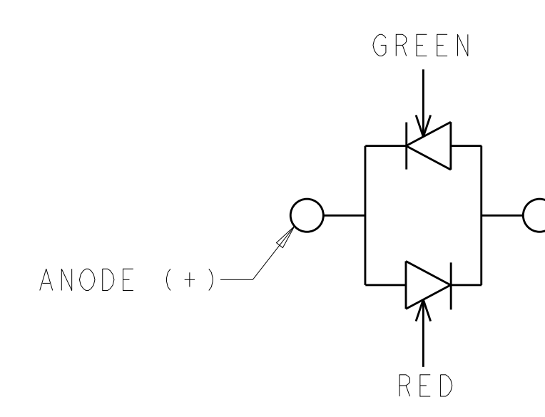
LED CIRCUIT DIAGRAM 6368062-6
