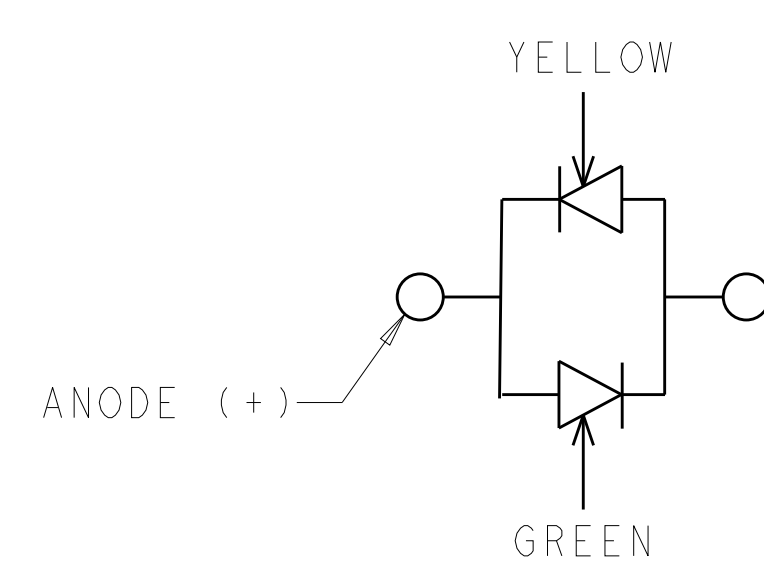
LED CURRENT DIAGRAM 6368062-4, -7
