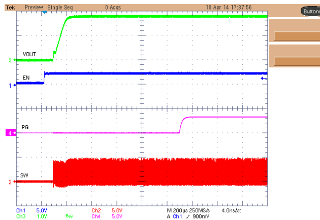
Figure 14. Power Up Sequence and Power Good ( V_{IN} = 3.6\text{ V} , V_{OUT} = 1.8\text{ V} , I_{OUT} = 0\text{ A} , L = 1\text{ }\mu\text{H} , C_{OUT} = 10\text{ }\mu\text{F} )
