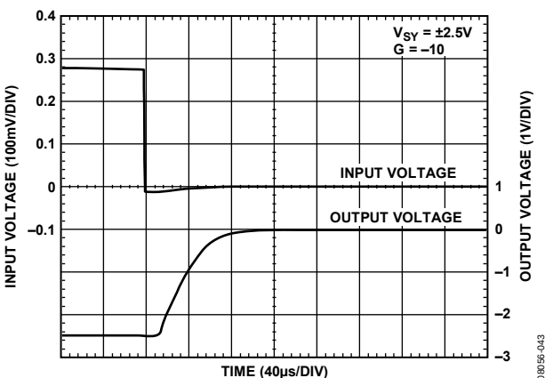
Figure 46. Positive Overload Recovery
