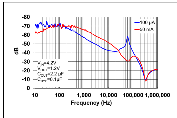
FIGURE 2-11: Power Supply Rejection Ratio (LDO1 LowQ Mode).
