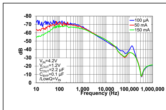
FIGURE 2-12: Power Supply Rejection Ratio (LDO1 Normal Mode).
