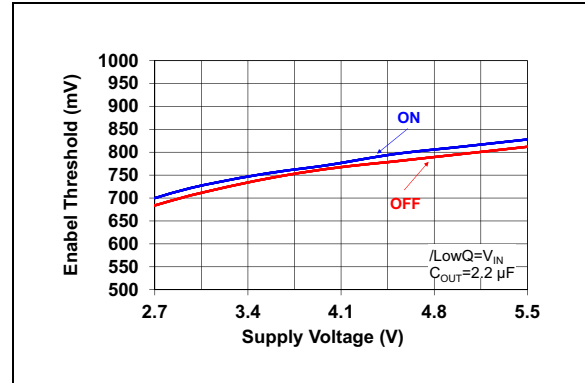
FIGURE 2-4: DC/DC Enable Threshold vs. Supply Voltage.
