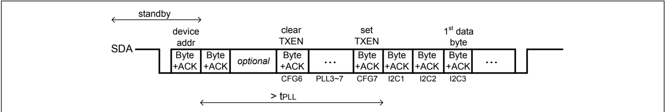
Figure 12. Using a Single I 2 C Transaction to Start Data Transmission From the Standby State
