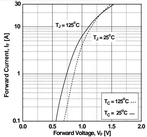
Figure 18. Forward Characteristics
