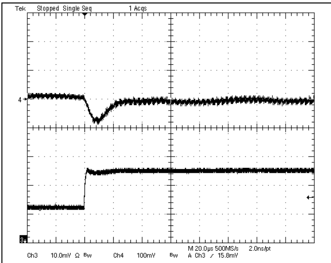
Fig-1.2V-6: Output voltage response for V_{out}=1.2V to positive load current step change from 2.5A to 5A with slew rate of 5A/\mu s at V_{in}=12V . C_o=47\mu F \times 2 ceramic.
