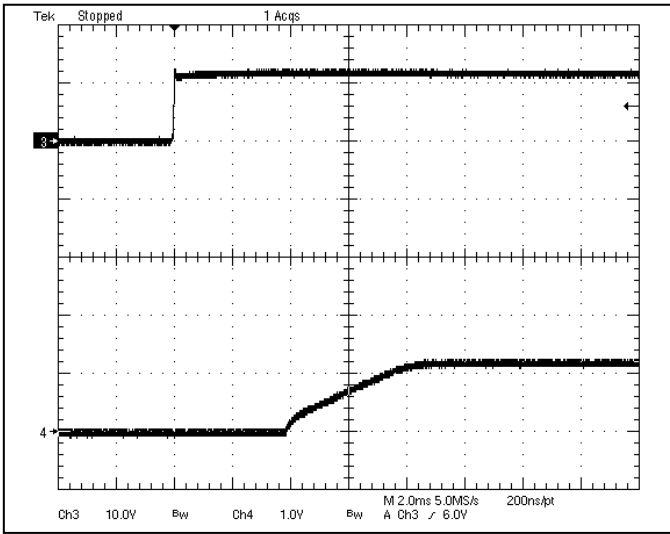
Fig-1.2V-4: Turn-on transient for V_{out}=1.2V with application of V_{in} at full rated load current (resistive) and 47\mu F \times 2 external capacitance at V_{in}=12V .
