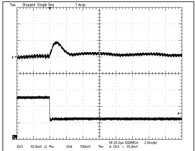
Fig-1.2V-7: Output voltage response for V_{out}=1.2V to negative load current step change from 5A to 2.5A with slew rate of -5A/\mu s at V_{in}=12V . C_o=47\mu F \times 2 ceramic.
