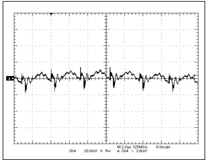
Fig-1.2V-5: Output voltage ripple (20mV/div.) for V_{out}=1.2V at full rated load current into a resistive load with external capacitance 47\mu F \times 2 ceramic + 1\mu F ceramic at V_{in}=12V .
