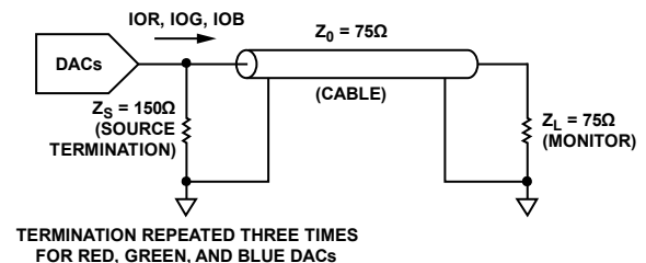
Figure 7. Analog Output Termination for RS-170
