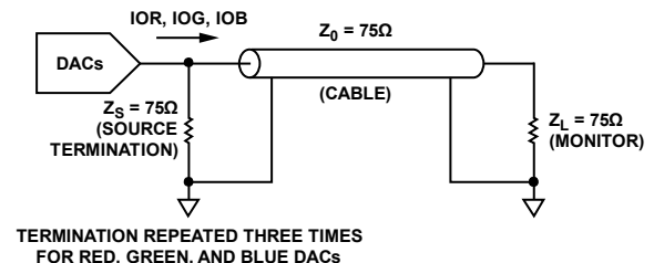
Figure 6. Analog Output Termination for RS-343A
