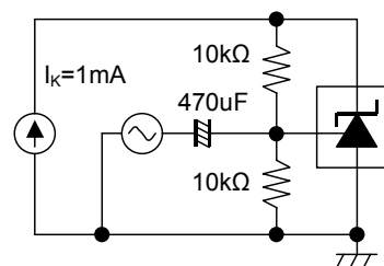
Fig.4 Gain and Phase to test circuit
