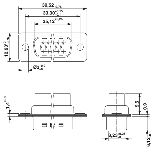
Dimensioned drawing
