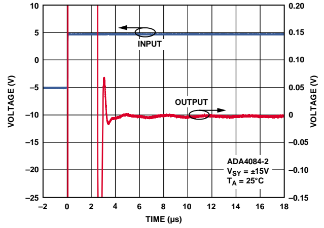
Figure 70. Settling Time
