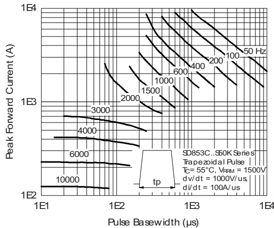
Fig. 20 - Frequency Characteristics
