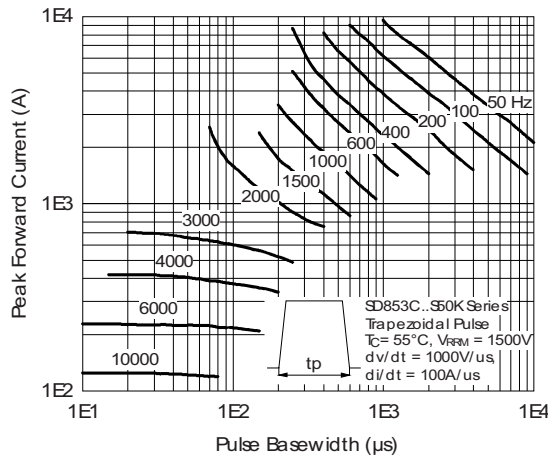
Fig. 20 - Frequency Characteristics
