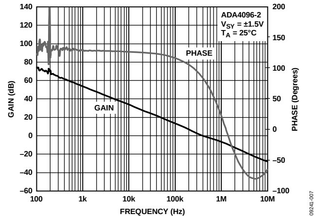
Figure 12. Open-Loop Gain and Phase vs. Frequency
