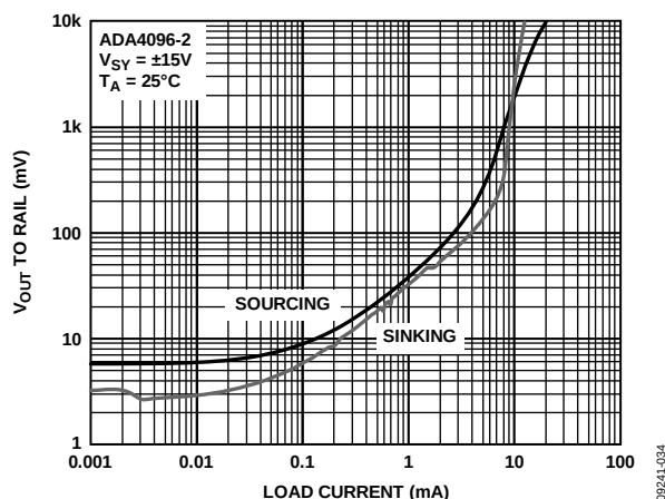
Figure 35. Dropout Voltage vs. Load Current
