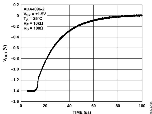
Figure 19. Negative Overload Recovery
