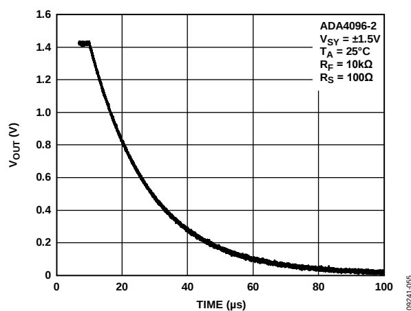
Figure 18. Positive Overload Recovery
