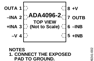
Figure 2. 8-Lead LFCSP (CP-8-10), ADA4096-2
