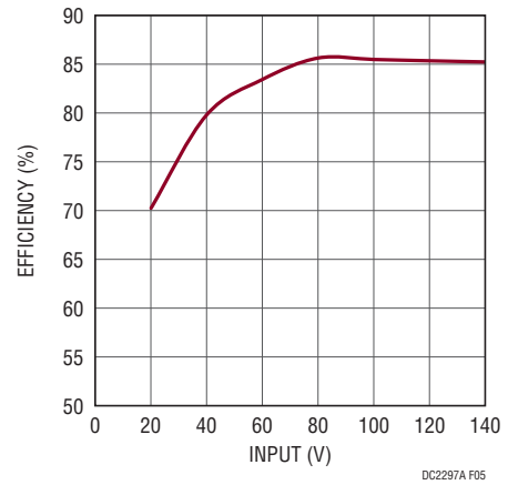
Figure 5. DC2297A-A Efficiency at 5V IN
