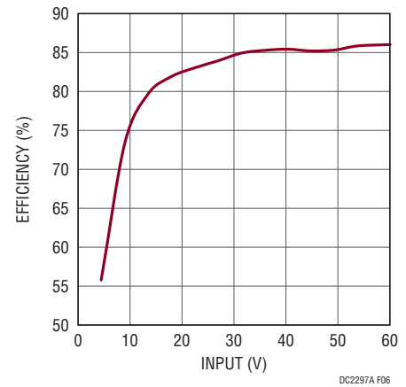
Figure 6. DC2297A-B Efficiency at 5V IN
