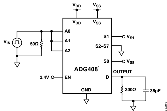
Figure 22. Switching Time of Multiplexer, t_{\text{TRANSITION}}
