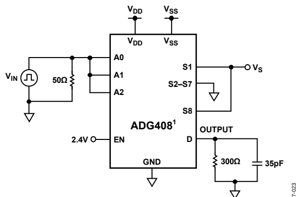
Figure 23. Break-Before-Make Delay, t_{\text{OPEN}}
