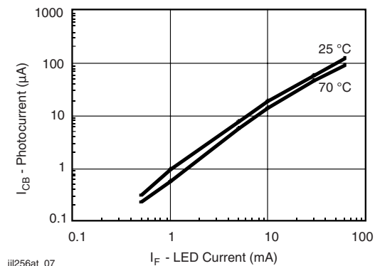
Figure 7. Photocurrent vs. LED Current
