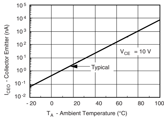
Figure 12. Collector-Emitter Leakage Current vs. Temp.
