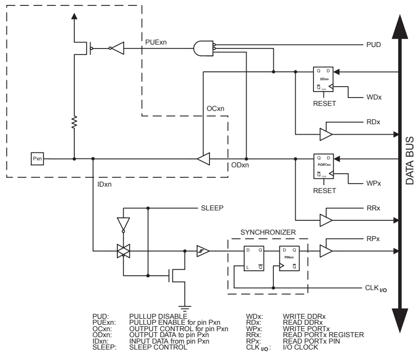
Figure 29-6. General Port Pin Schematic diagram
