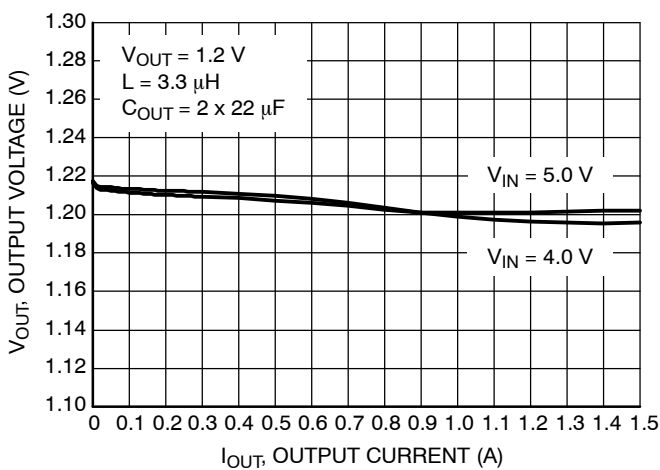
Figure 13. Load Regulation for V_{OUT} = 1.2\text{ V}
