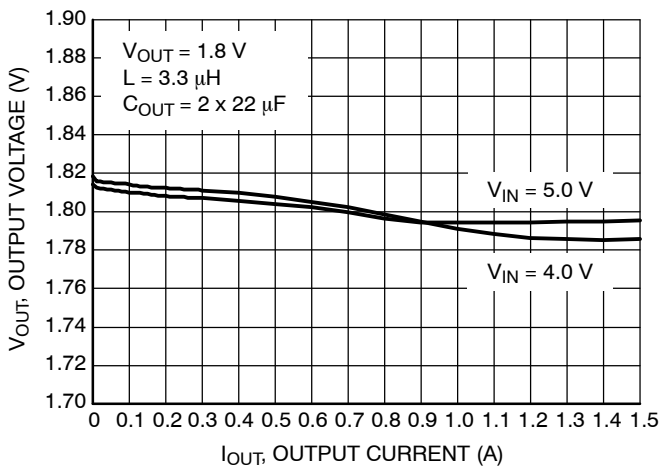
Figure 11. Load Regulation for V_{OUT} = 1.8\text{ V}
