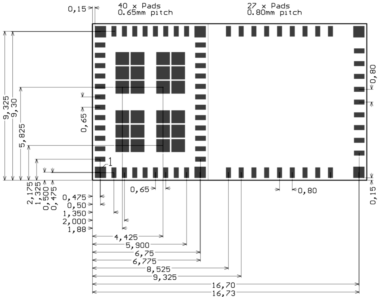
Bottom view
