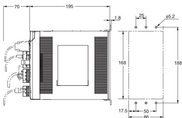
Mounting dimensions
