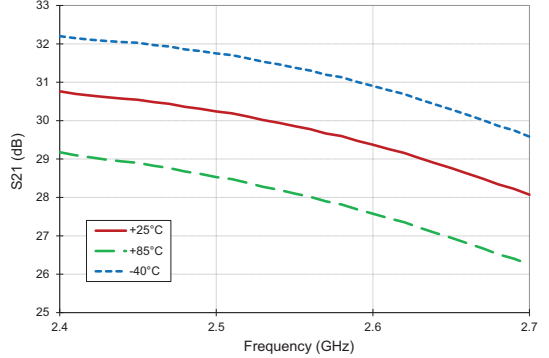
Gain versus Frequency and Temperature at 0dB Attenuation State
